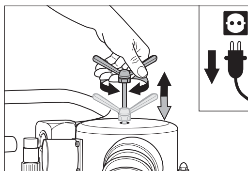
Fig. 61 Move the cleaning slide up and down while continuously turning the wing nut.
