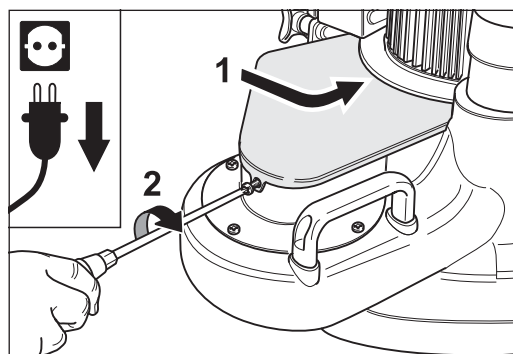
Fig. 100 Insert the V-belt guard into the slot at the motor, push it towards the motor (1) and tighten it with the screw (2).
