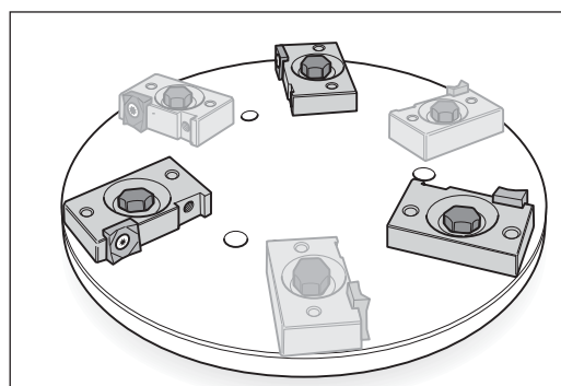
Fig. 37 You can use 3 or 6 holders on one milling disc. Each holder has to have at least one indexable insert!
