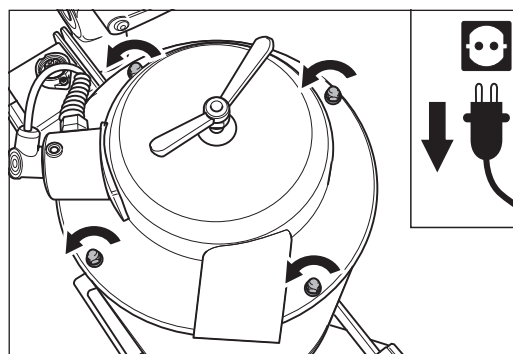
Fig. 67 Remove the four cap nuts and washers on top of the dust separator.
