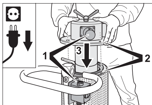
Fig. 72 Position the upper part of the separator (1 + 2) and insert it into the filter cartridge (3).
