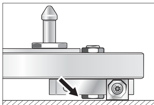
Fig. 39 Less aggressive adjustment of the milling disc with special screw for working depth turned out .
