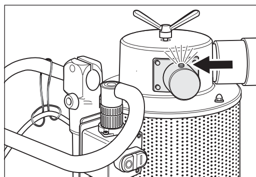
Fig. 60 If the red LED of the sensor lights up, check whether the dust bag is full and the filter cartridge should be cleaned!
