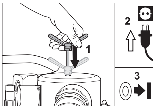
Fig. 62 Push the cleaning slide as deep as possible into the dust separator (1). Insert the power plug into the mains socket (2). You can now switch the machine back on again (3).
